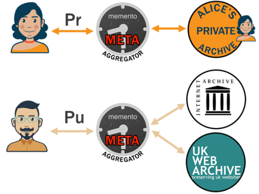
Figure 5: PrivateOnly and PublicOnly aggregation in an MMA.
